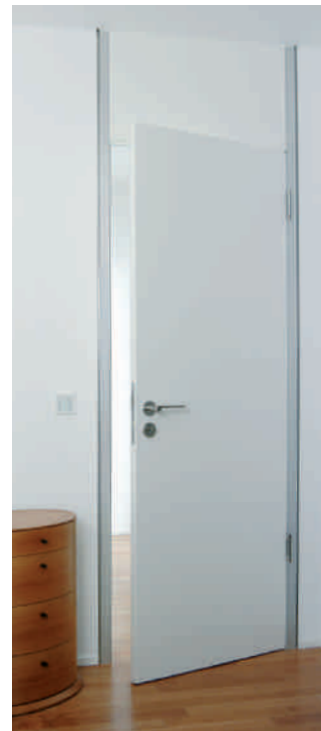
ULTRA-EXCLUSIV System PLANO Schleiflack weiß ähnl. RAL 9010 Oberblende in Türblattausführung Aluminiumzarge FLAT ULTRA-EXCLUSIV System PLANO White rubbed lacquer finish similar to RAL 9010 Fanlight matching door leaf design Aluminium frame-FLAT
